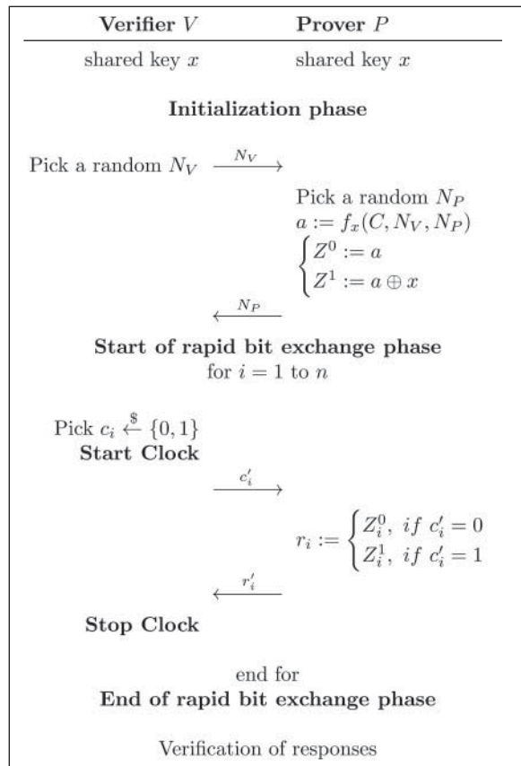
FIGURE 1. A general view of the distance-bounding protocols proposed in [7–10].
