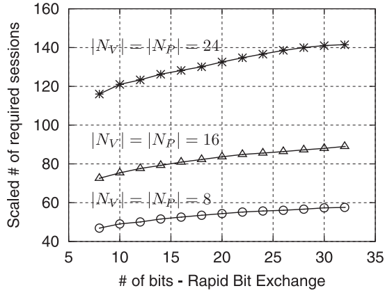
FIGURE 2. Expected number of required sessions for ideal communication channel ( \text{BER} = 0.0 ) for various nonce lengths m as the number of rounds n and the key length k = n increase. Note that the number of sessions is scaled down by 10 and 100 for m = 16 and m = 24 , respectively.
